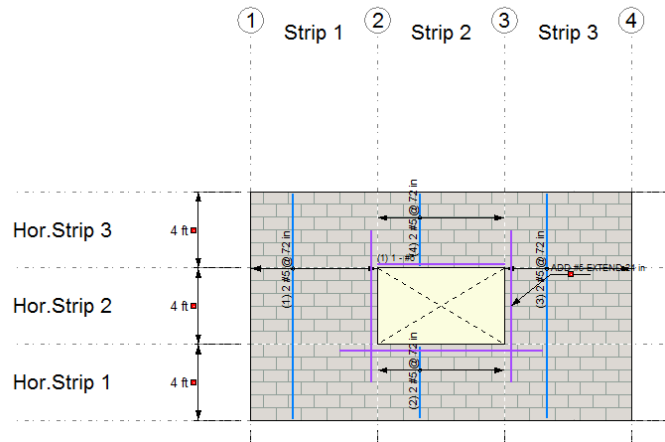
Figure 5: image above from RISA showing wall areas, image to the right of RAM Elements showing wall strips
