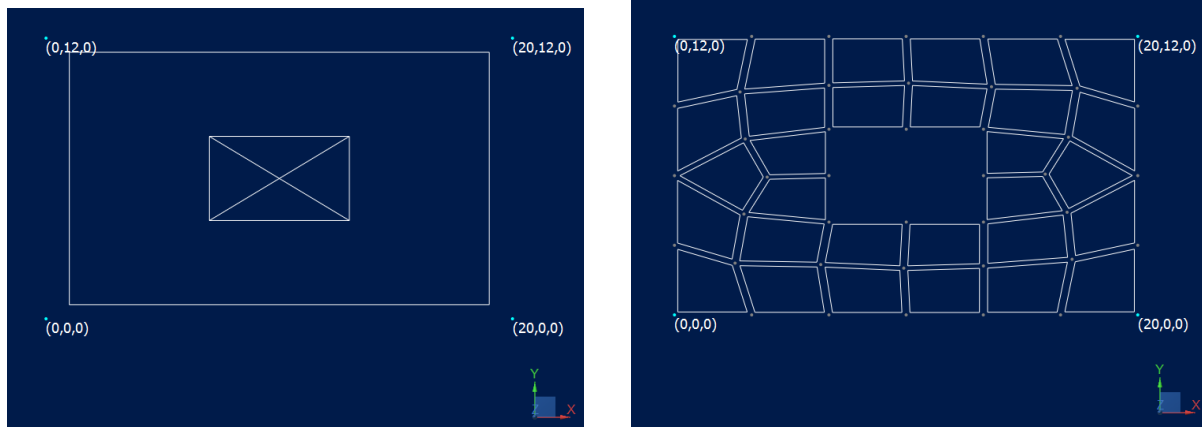
Figure 3: Wall Geometry with opening | Wall discretized into finite elements example of automatic meshing from RAM Elements
