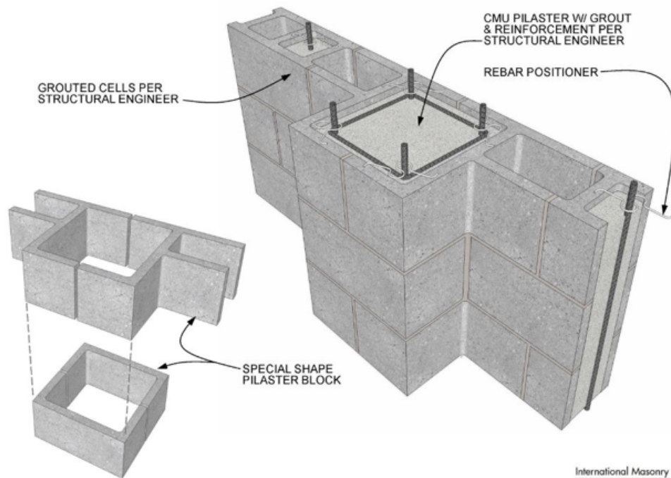
LOAD BEARING PILASTER DETAIL 02.010.1101 REV. 06/17/08
