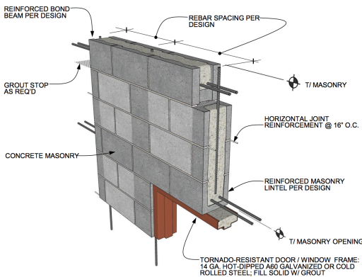
Figure 4: Storm Shelter Head Detail IMI Masonry Detail Series,
